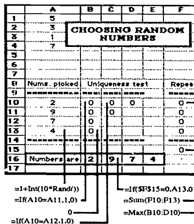
Figure 7. Choosing four natural numbers between one and ten
